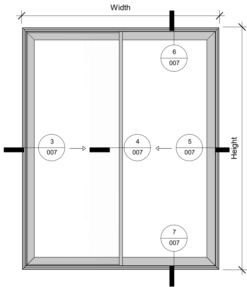
1 Elevation Front 1 : 20
